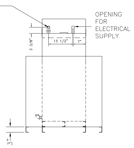
REAR VIEW
